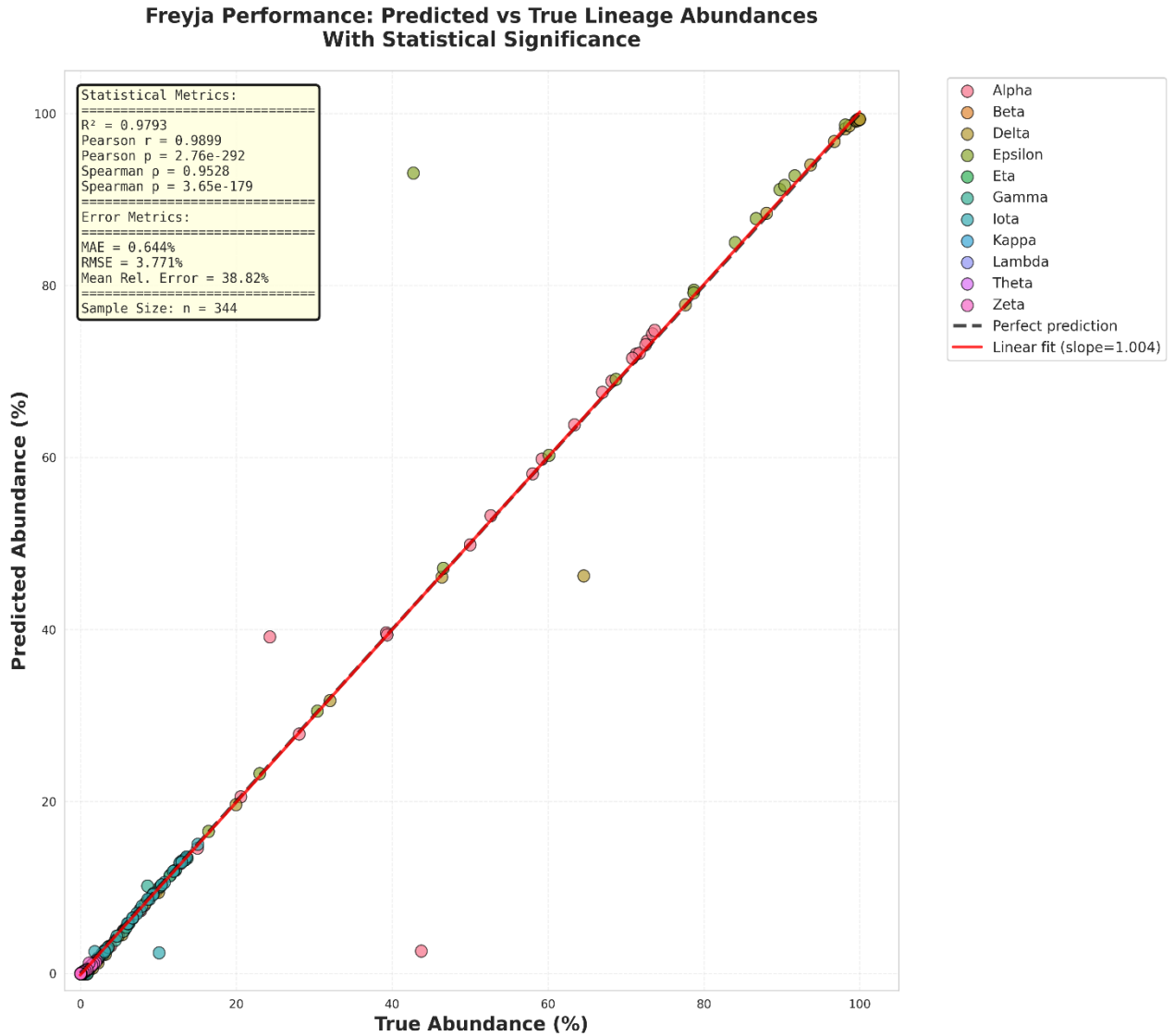
Figure 11. Performance of Freyja in comparing predicted and true SARS-CoV-2 lineage abundances
