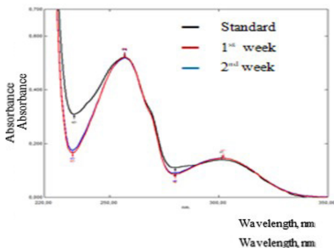
Fig. 5. Modification of the concentration of Dioxoindolinone following influence of humidity (1) and the absorption spectra of Dioxoindolinone under the influence of humidity (2)/
