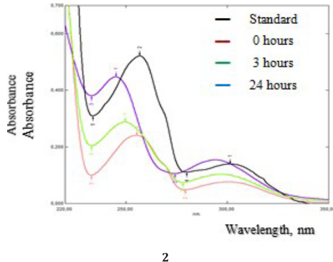
Fig. 4. Modification of the concentration of Dioxoindolinone following basic hydrolysis (1) and the absorption spectra of Dioxoindolinone under the action of basic hydrolytic stress (2)
