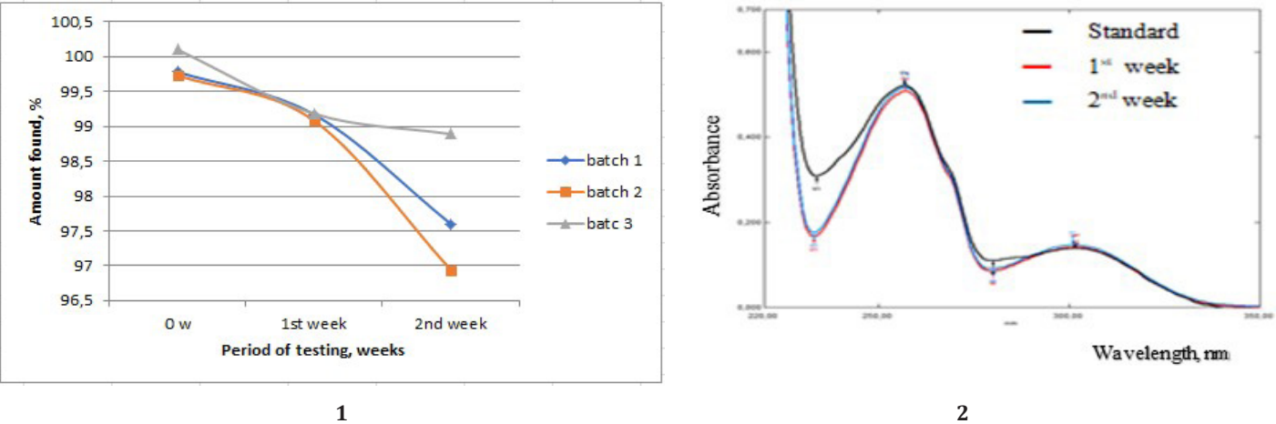
Fig. 7. Modification of the concentration of Dioxoindolinone following thermal stress (1) and the absorption spectra of Dioxoindolinone under the action of thermal stress (2)
