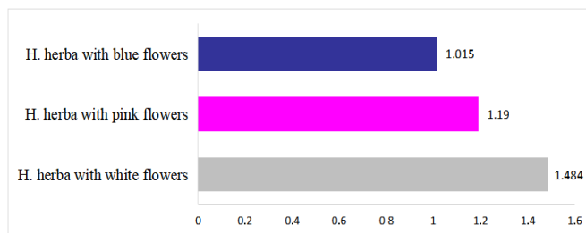
Fig. 2. The total content of hydroxycinnamic acids in plant products from the aerial parts of Hyssopus officinalis L. (mg/g)
